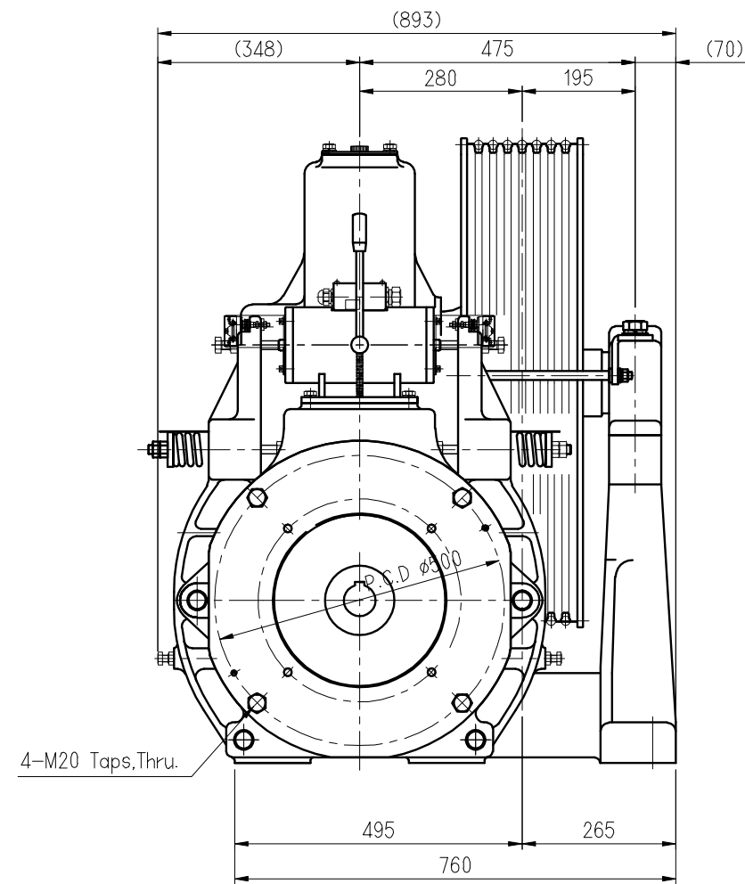
View "A"
