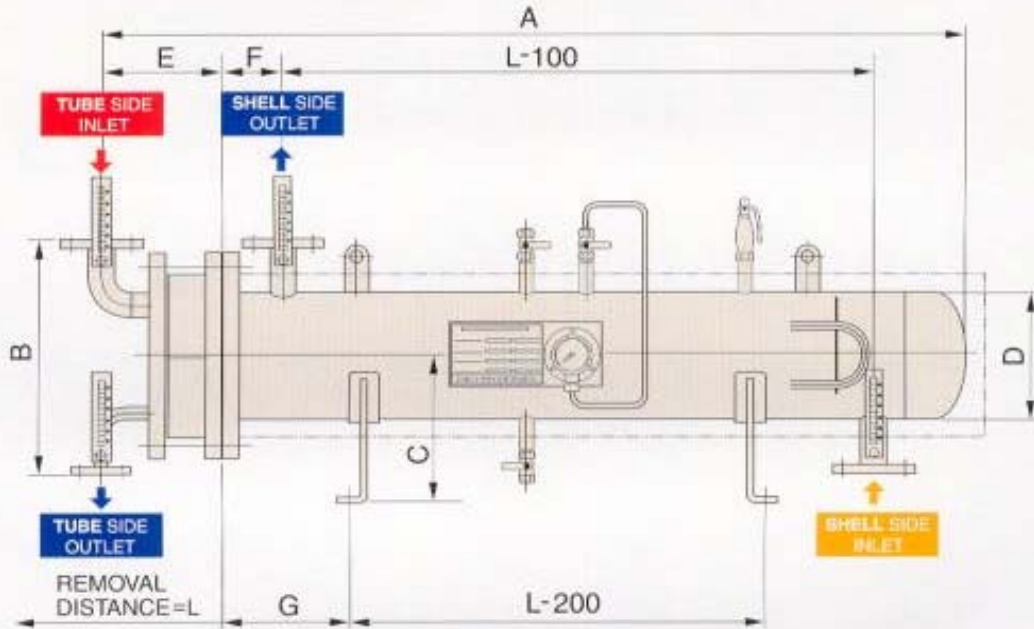
Outline Dimension (mm)
