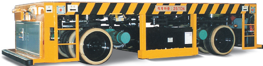
▲ 4-WHEEL DRIVE AND 4-WHEEL STEERING TYPE WITH SMALL TURNING RADIUS SUITABLE FOR TURNING IN THE NARROW PASSAGEWAY
