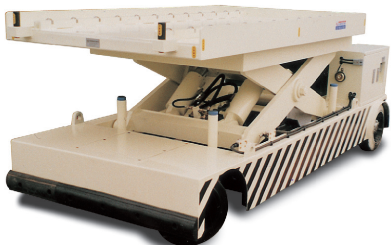
◀ ELECTRIC SCISSOR TRACKLESS TRANSPORTER CAR MANUFACTURED AND DELIVERED TO LG ELECTRONICS
