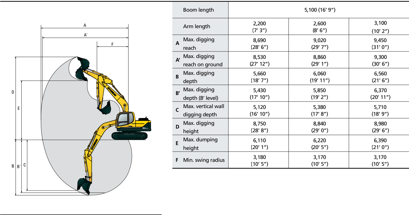
R160LC-9 WORKING RANGE
