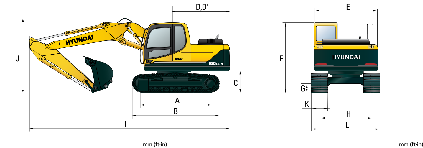
R160LC-9 2-PIECE BOOM DIMENSIONS
