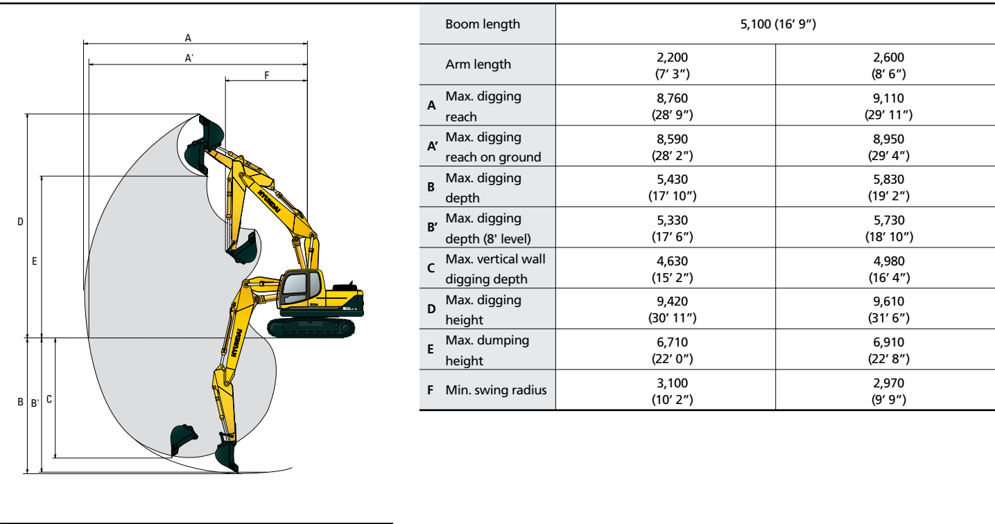
R160LC-9 2-PIECE BOOM WORKING RANGE
