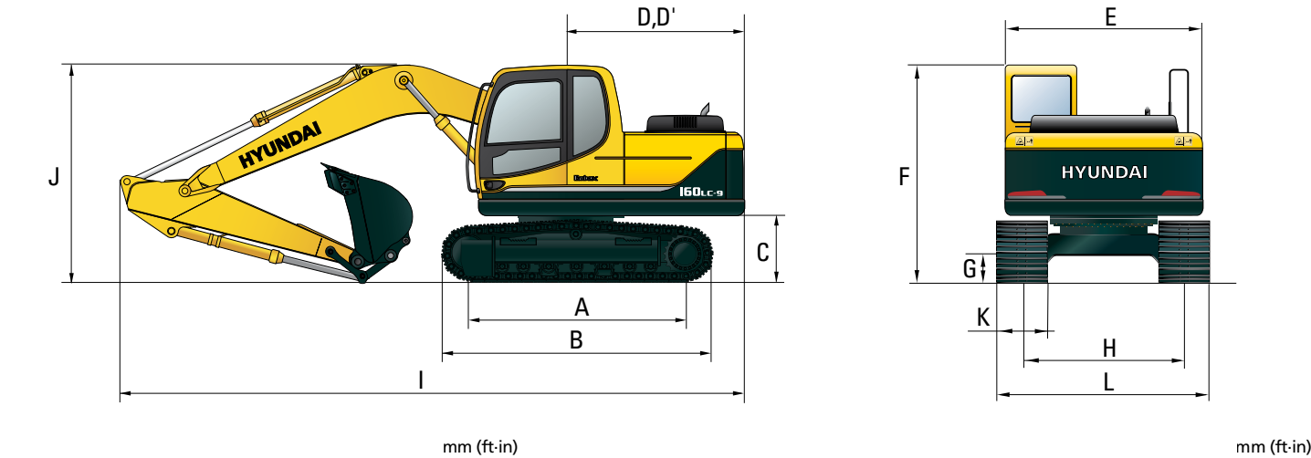
R160LC-9 DIMENSIONS
