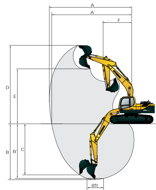
R300NLC-9S (9SH) WORKING RANGE
