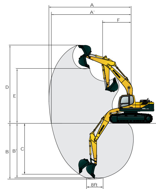
R300LC-9S / 9SH HIGH WALKER WORKING RANGE
