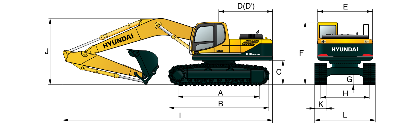
R300NLC-9S (9SH) DIMENSIONS
