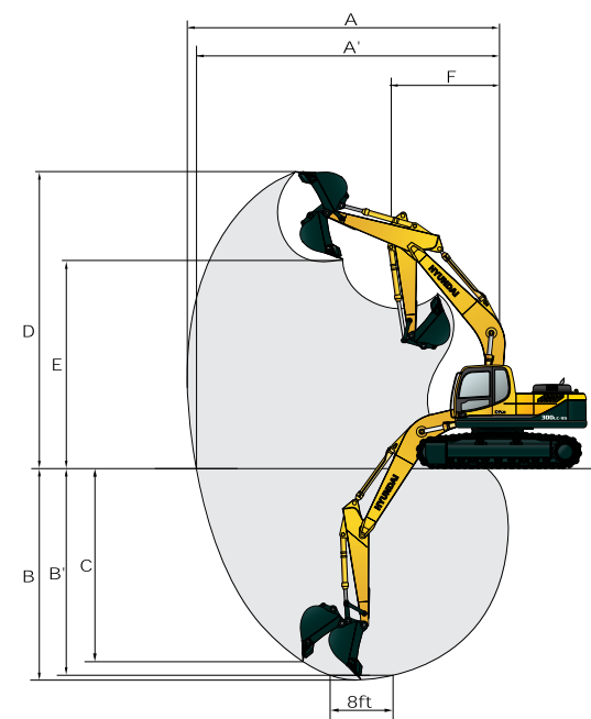
R300LC-9S (9SH) WORKING RANGE
