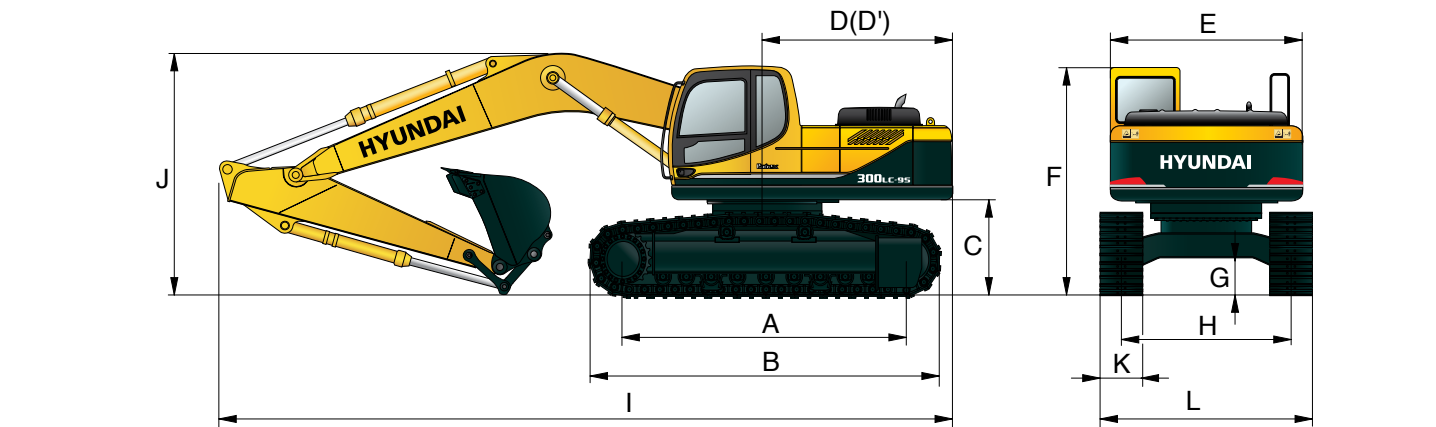
R300LC-9S / 9SH HIGH WALKER DIMENSIONS
