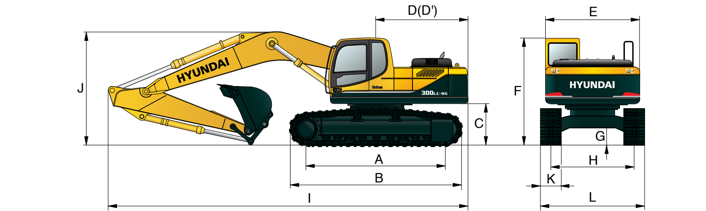
R300LC-9S (9SH) DIMENSIONS
