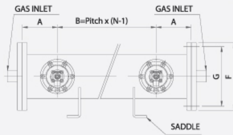
FLANGE TYPE
