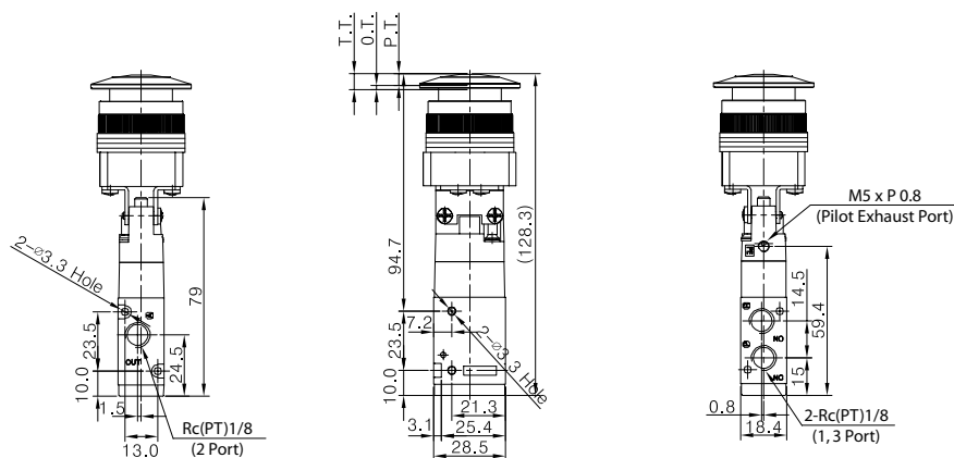
Push Button (Flat type) KVM 341-01-33
