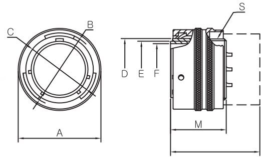
Termination Assembly
