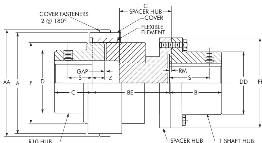
SPACER DIMENSIONS — MILLIMETERS
