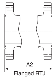
Flanged RTJ
