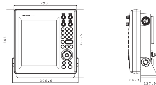
ECHO SOUNDER SES-3000(N)
