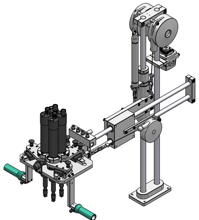
BA 200 with multi spindle and variable pitch.
