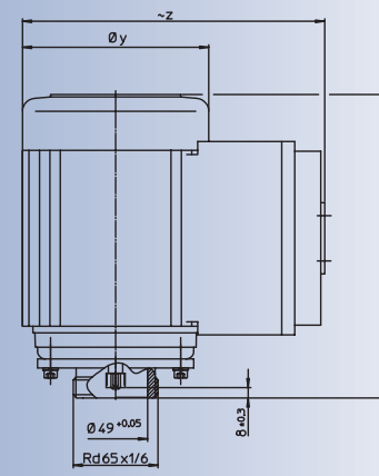
Single-phase motor (SPM) with capacitor switch, for use with F 550 GS6 and F 520 S-41/37
