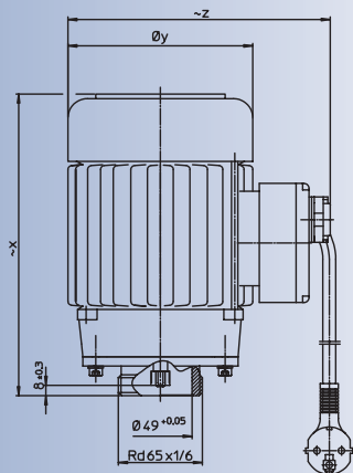
Single-phase motor (SPM) with capacitor switch, for use with F 550 GS6 and F 520 S-41/37
