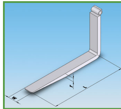
TINE
