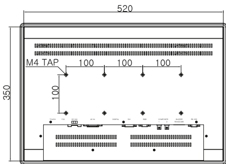
REAR VIEW
