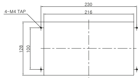
PANEL CUTTING
