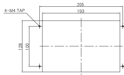
PANEL CUTTING
