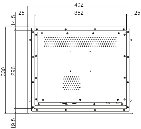
REAR VIEW
