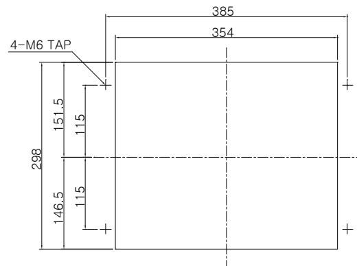
PANEL CUTTING
