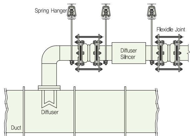
Conceptual diagram of vibration and noise reduction measures using diffuser type acoustic silencer
