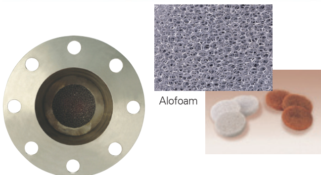
Diffuser type acoustic silencer product quality
