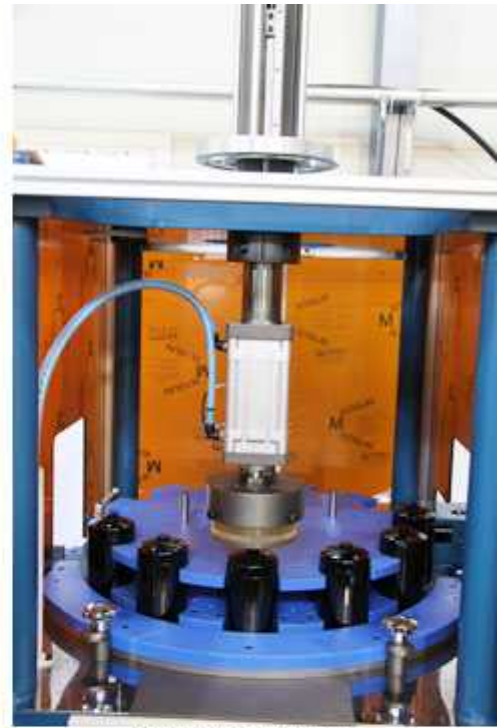
SEAMING POCKET
