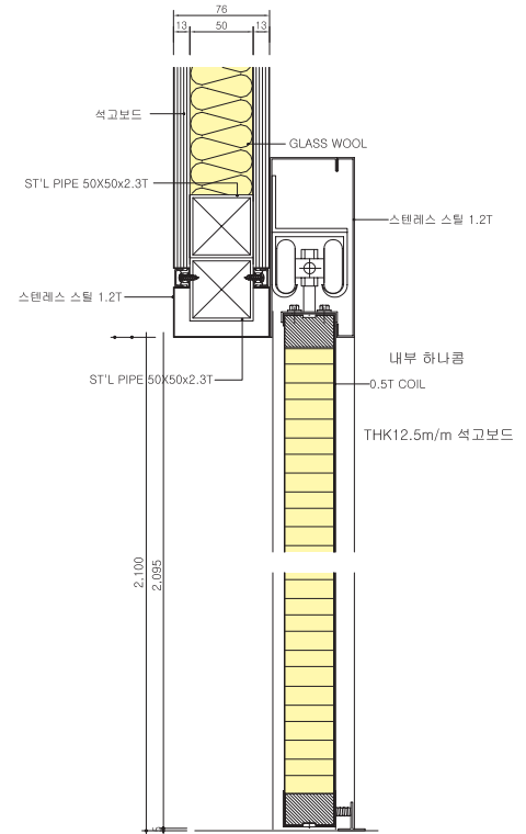
SECTION-B
