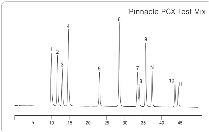
Carbamate Chromatogram
