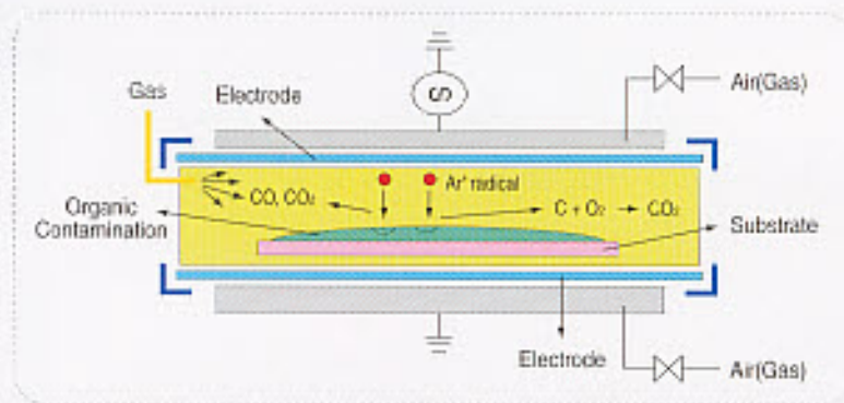
Schematic Diagram for Vacuum Plasma
